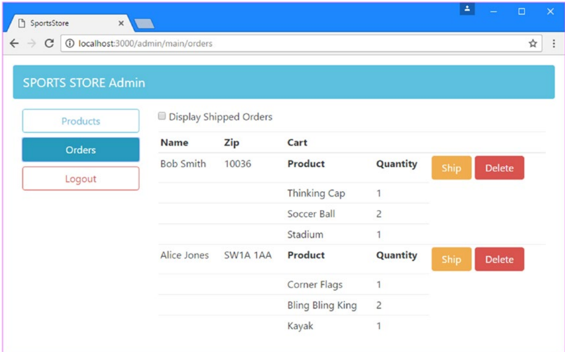
Figure 9-7. Managing orders
