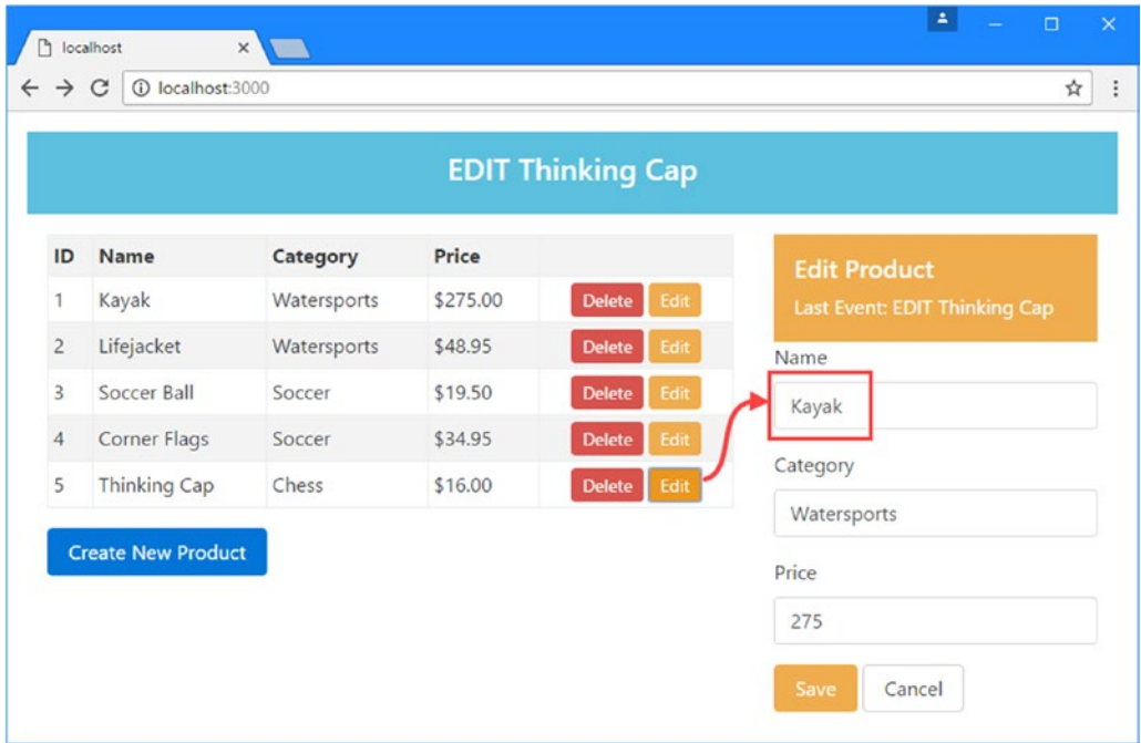
Figure 23-9. Transforming events
