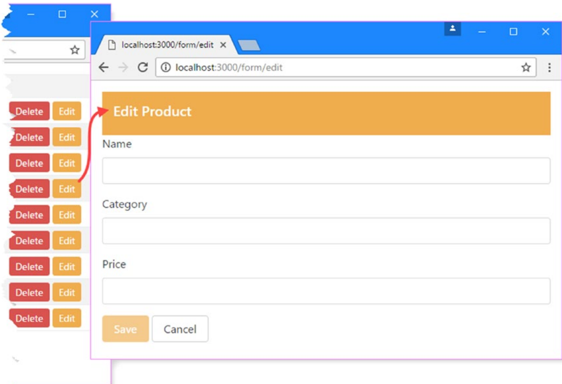
Figure 25-4. Using the active route in a component
